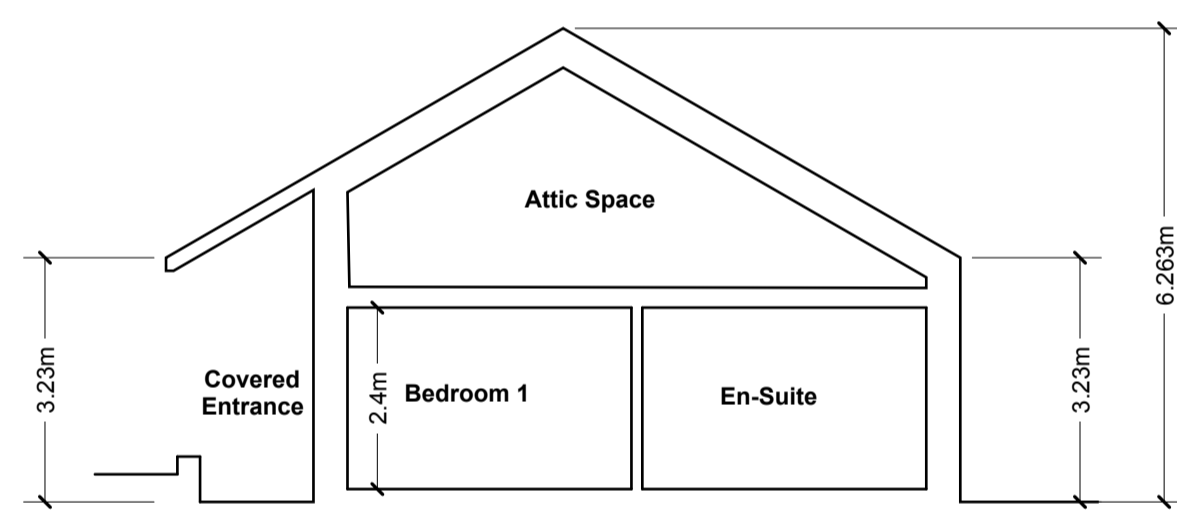
SECTION B
