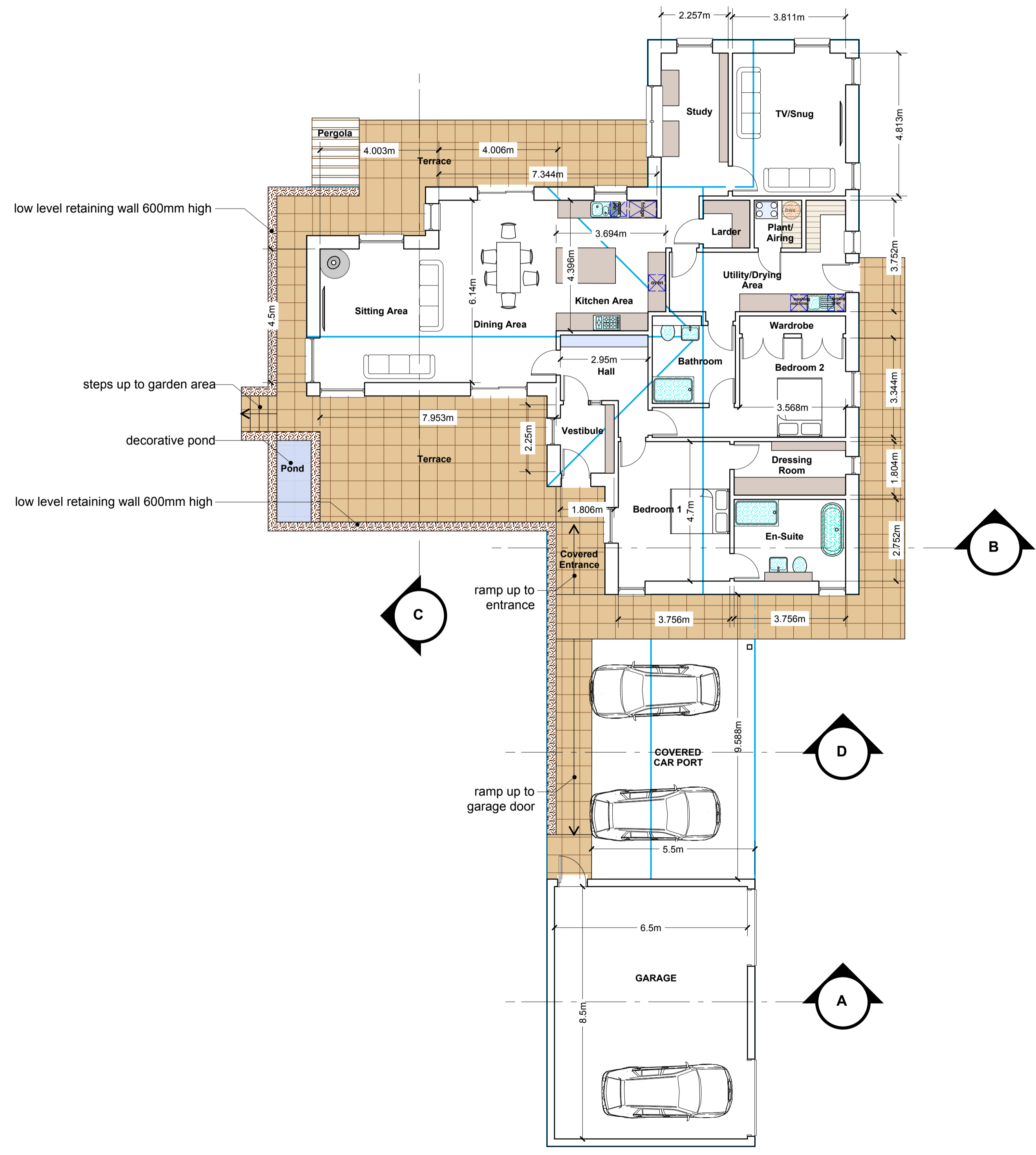
FLOOR PLAN
