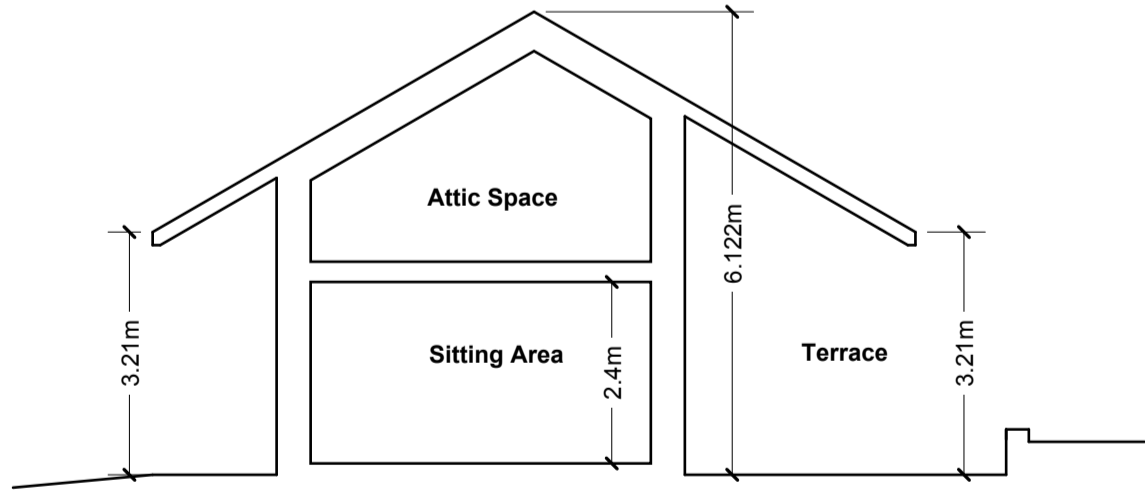
SECTION B
