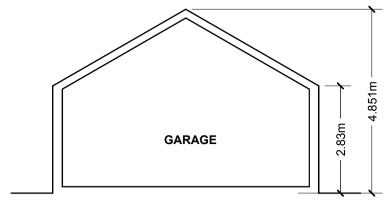
SECTION A
